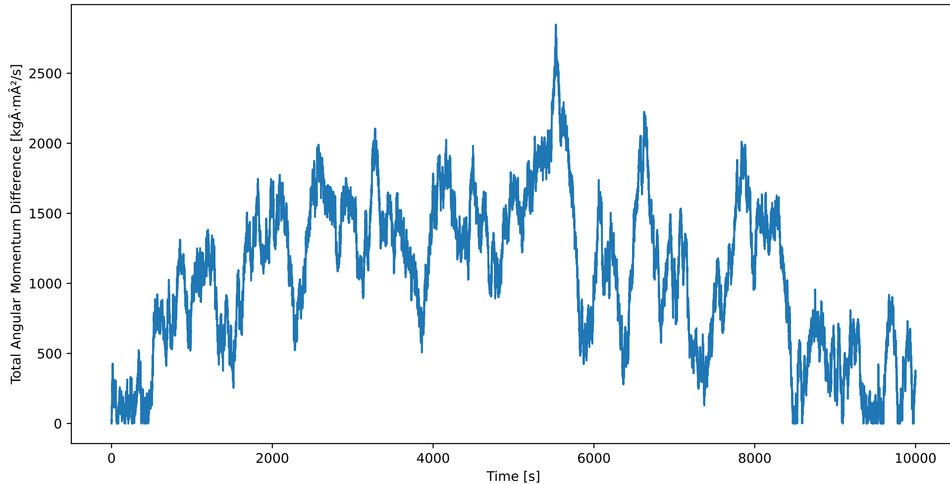
Total Angular Momentum Drift over time
